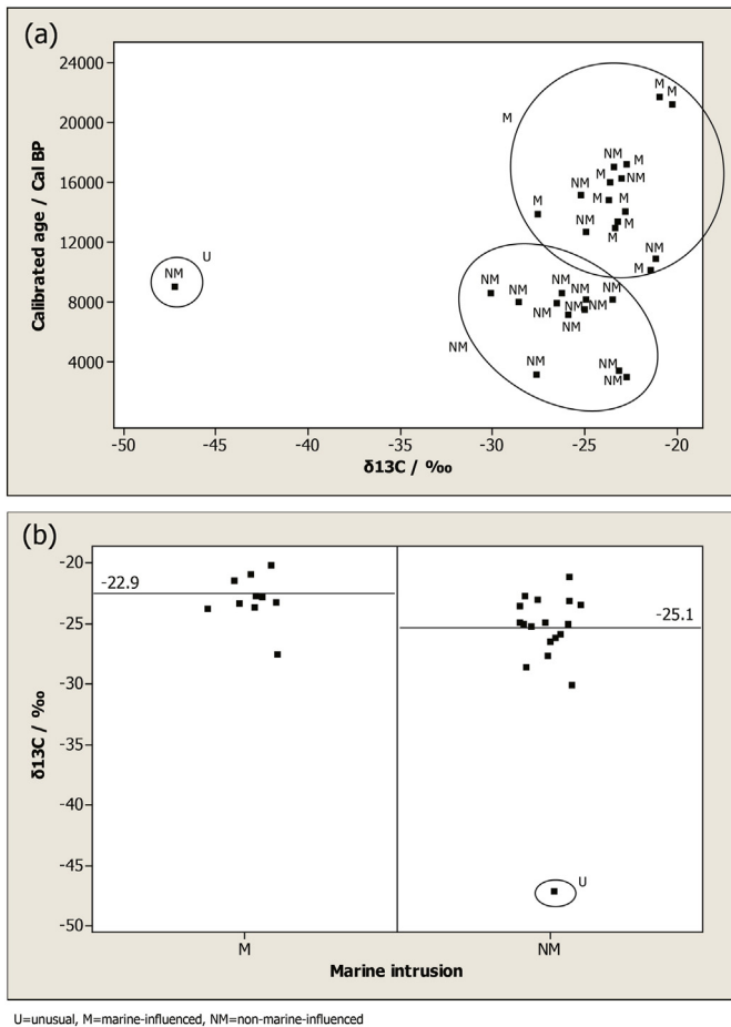
Fig. 3. The \delta^{13}\text{C} values of ^{14}\text{C} samples in sediment sequences from the southern Yangtze Delta: (a) \delta^{13}\text{C} values versus measured age, where pre-Holocene dating anomalies are found in association with marine influences – except a minor proportion of unusual samples. The circle marked with M indicates where marine-influenced samples cluster, whereas the circle marked with NM indicates where non-marine-influenced samples cluster. An unusual sample (dated on organic-rich mud) is identified given its unusual \delta^{13}\text{C} value. (b) \delta^{13}\text{C} values of marine-influenced samples and non-marine-influenced samples, where marine-influenced samples (labelled according to microfossil evidence) are found with systemically higher \delta^{13}\text{C} values than non-marine-influenced samples. The two lines, -25\% and -23\% in value, represent an average of \delta^{13}\text{C} values of all samples in, respectively, the non-marine-influenced and marine-influenced assemblage. Therefore \delta^{13}\text{C} values actually provide an independent line of evidence to confirm results from microfossil evidence.
