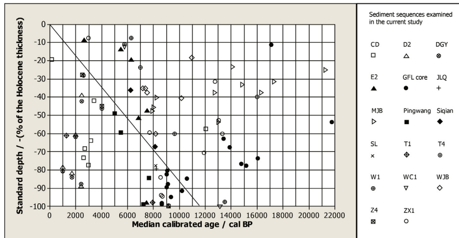
Fig. 2. Median calibrated age plotted versus standardised depth of ^{14}\text{C} data in 17 Holocene-aged sediment sequences recovered from the southern Yangtze Delta, China. The figure primarily shows temporal differences in occurrence of ^{14}\text{C} dates. Data from a same sequence use a same symbol; therefore 17 different symbols are used to represent the 17 sequences: CD (Long et al., 2014), D2 (Stanley and Chen, 2000), DGY (Zhao et al., 2007), E2 (Wang et al., 2001), GFL core (Wang et al., 2012), JLQ (Stanley and Chen, 2000), MJB (Long et al., 2014), Pingwang (Zong et al., 2011), Siqian (Zong et al., 2011), SL (Stanley and Chen, 2000), T1 (Stanley and Chen, 2000), T4 (Stanley and Chen, 2000), W1 (Wang et al., 2001), WC1 (Stanley and Chen, 2000), WJB (Qin et al., 2011), Z4 (Stanley and Chen, 2000), and ZX1 (Stanley and Chen, 2000). The diagonal line on the plot represents a baseline of a constant sedimentation rate. The standardised depth of a ^{14}\text{C} sample is calculated as a proportion of the actual depth of that sample to the total thickness of the Holocene in the sequence which the sample is collected from.
